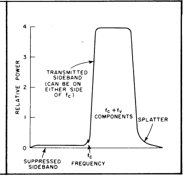
Figure 4: single sideband.
