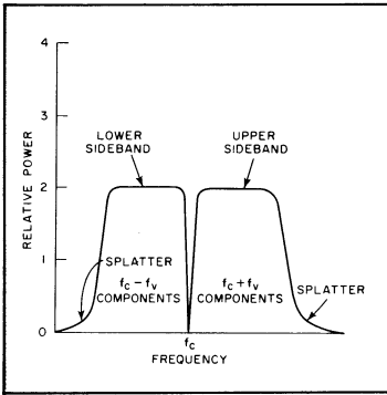
Figure 2: double sideband.
