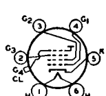
-D- ULTOR = G_4 + CL FOCUSING ELECTRODE = G_2
