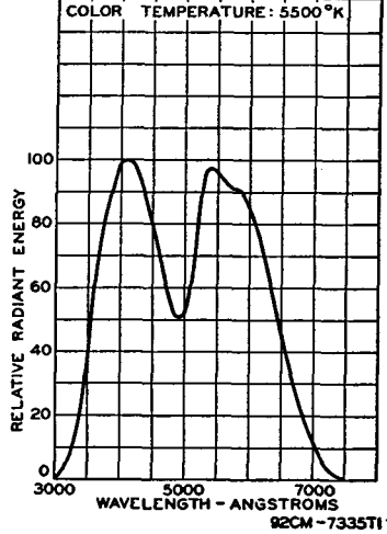
SPECTRAL-ENERGY EMISSION CHARACTERISTIC OF PHOSPHOR P4 SILICATE TYPE
