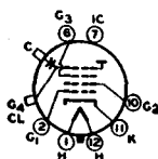
-B- ULTOR = G_4 + CL FOCUSING ELECTRODE = G_2
