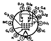
-C- ULTOR = G_2 + G_4 + CL FOCUSING ELECTRODE = G_2
