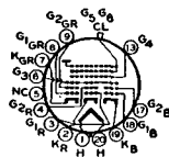
-K- ULTOR = G_5 + G_6 + CL FOCUSING ELECTRODE = G_2
