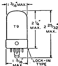
INTERMEDIATE- SHELL OCTAL
