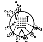
-H- ULTOR = G_2 + G_3 + CL FOCUSING ELECTRODE = G_2
