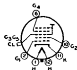
-G- ULTOR = G_2 + G_3 + CL FOCUSING ELECTRODE = G_2
