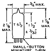
SMALL-BUTTON MINIATURE 7-PIN
