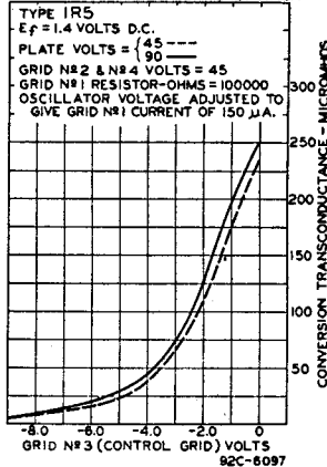
OPERATION CHARACTERISTICS WITH SEPARATE OSCILLATOR EXCITATION
